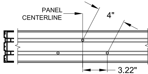
2-TRACK INTERMEDIATE "+3" ANCHOR LOCATIONS
