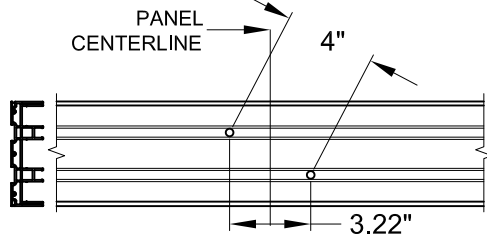
2-TRACK INTERMEDIATE "+2" ANCHOR LOCATIONS
