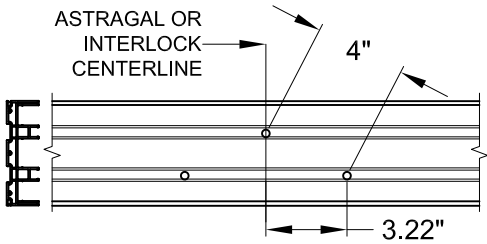
2-TRACK CLUSTER "C3" ANCHOR LOCATIONS
