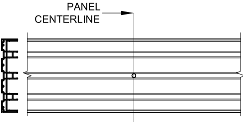
3-TRACK INTERMEDIATE "+1" ANCHOR LOCATION
