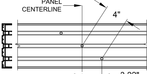
3-TRACK INTERMEDIATE "+3" ANCHOR LOCATIONS
