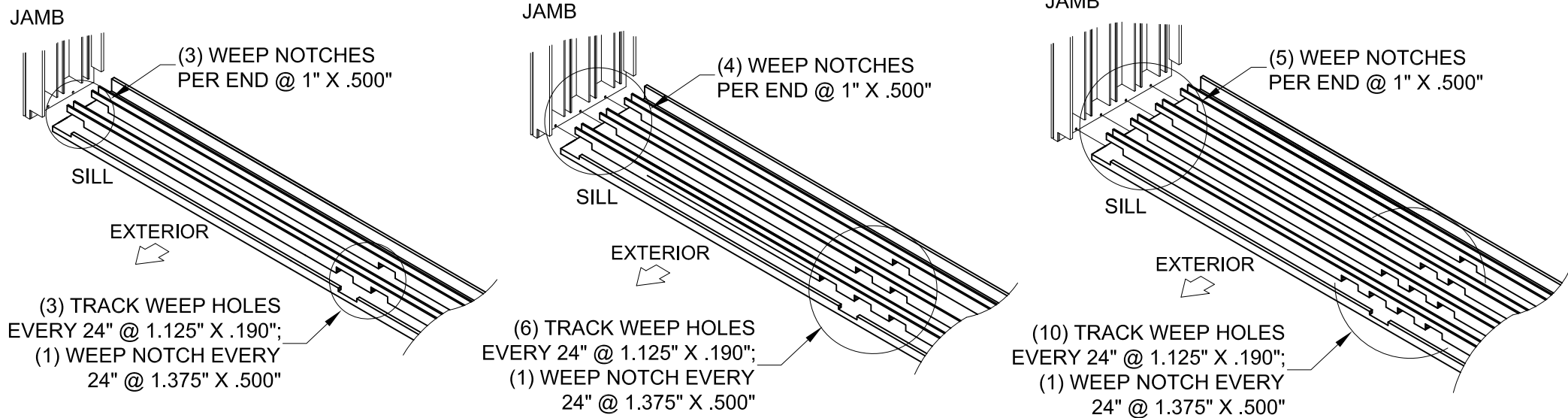
SILL WEEPHOLE LAYOUT (2, 3 & 4 TRACKS)
