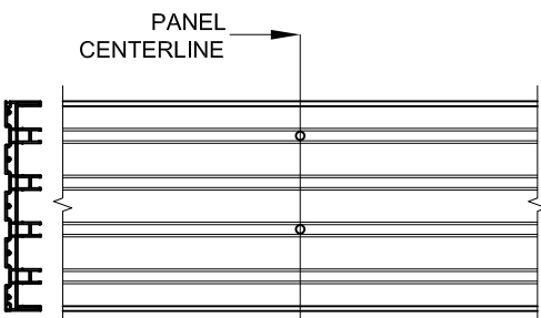
4-TRACK INTERMEDIATE "+2" ANCHOR LOCATIONS
