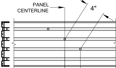
4-TRACK INTERMEDIATE "+3" ANCHOR LOCATIONS
