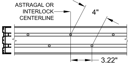
2-TRACK CLUSTER "C5" ANCHOR LOCATIONS
