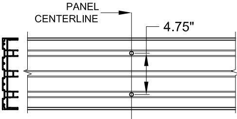
3-TRACK INTERMEDIATE "+2" ANCHOR LOCATIONS
