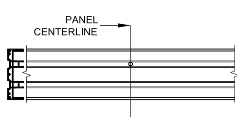
2-TRACK INTERMEDIATE "+1" ANCHOR LOCATION
